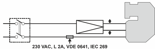
Fig. 4. Electric wiring of motor
